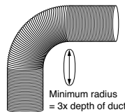
Figure 2. 90° Lateral bend
