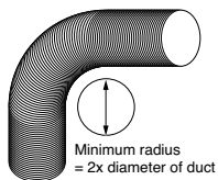
Figure 1. 90° bend
